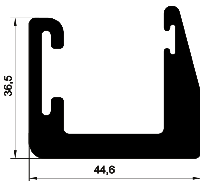
EIR-033 5,166 kg/m
