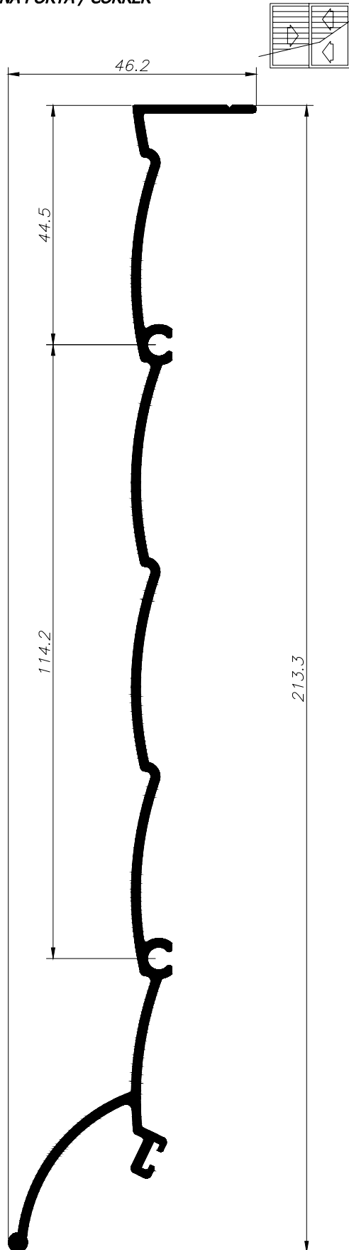
TAMPA EXTERNA PORTA / CORRER
