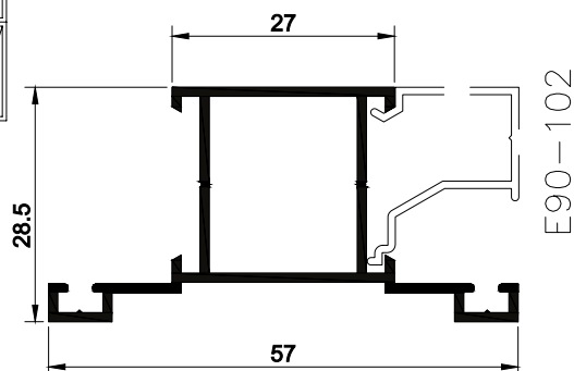
COLUNA / MAXIM-AR
