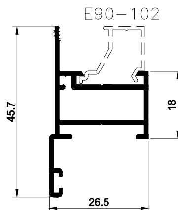
TRAVESSA / MAXIM-AR
