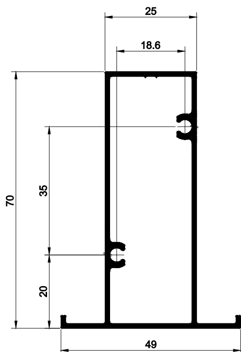
COLUNA
