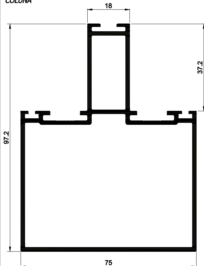
COLUNA
