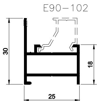
TRAVESSA SUPERIOR / MAXIM-AR
