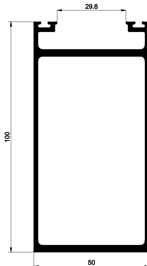
COLUNA
