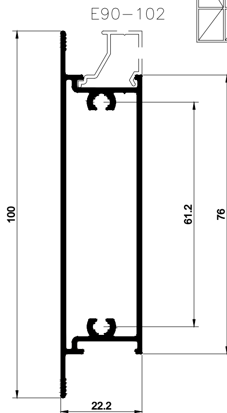
TRAVESSA CENTRAL / CORRER E GIRO
